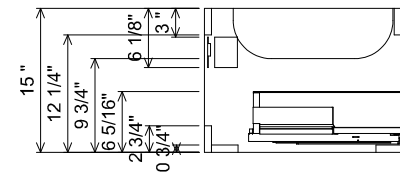
AT SINK CENTER SECTION
