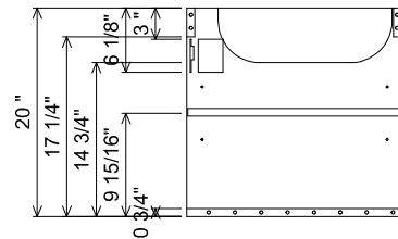
AT WING SECTION
